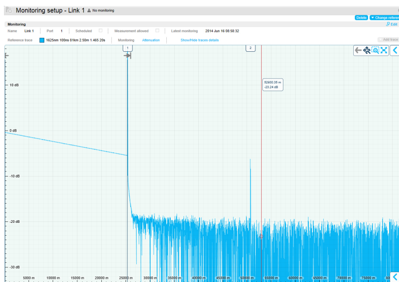
Figure 9 Reference Trace
