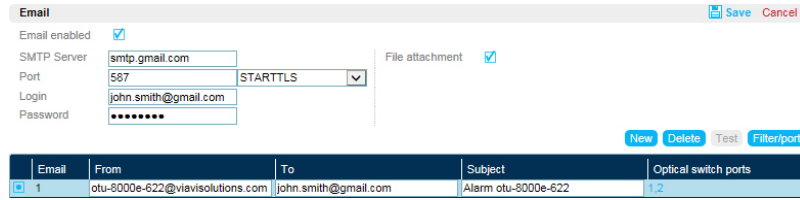
Figure 40 Example of email configuration with Gmail
